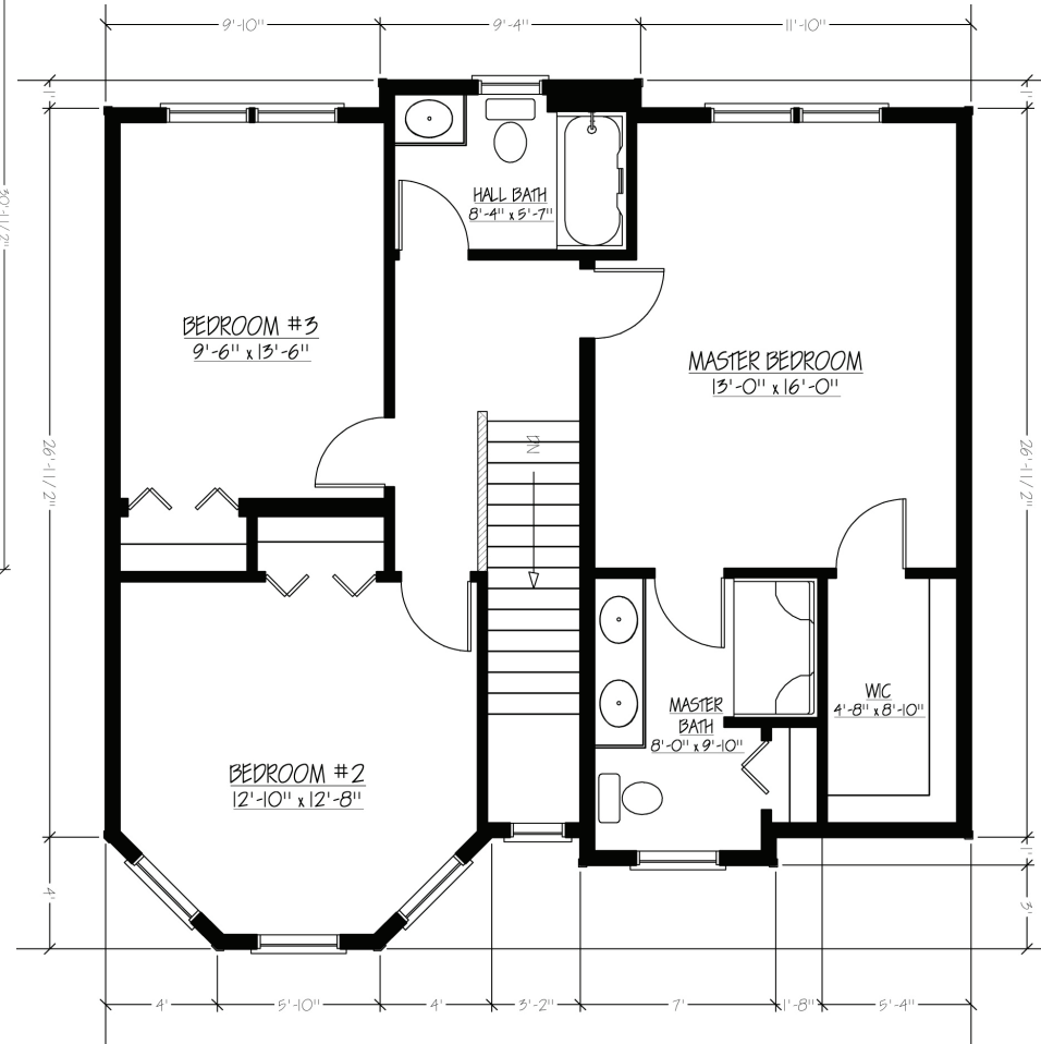
Second Floor
